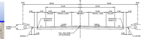
TYPICAL SECTION
